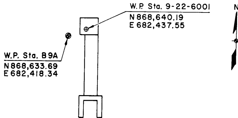
Fig. 2—Plan, Area 9 structure.
